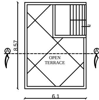
FLOOR-FIRST TERRACE FLOOR PLAN
