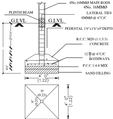
FOUNDATION DETAIL
