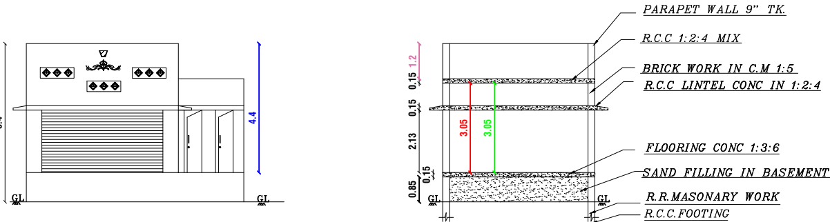
FRONT ELEVATION
