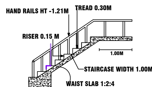
STAIRCASE DETAILS
