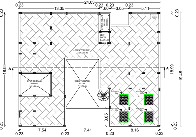
FLOOR - TERRACE PRO.TERRACE FLOOR PLAN
