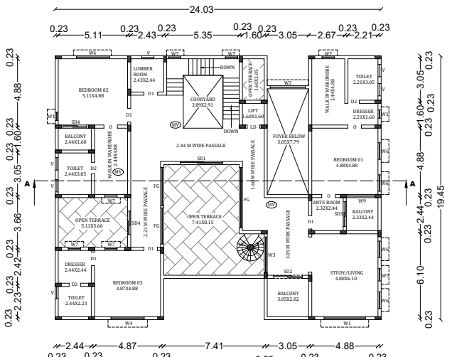
FLOOR - FIRST PRO.FIRST FLOOR PLAN
