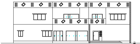
ELEVATION (EAST SIDE)
