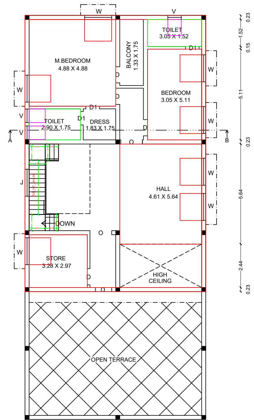
FIRST FLOOR
