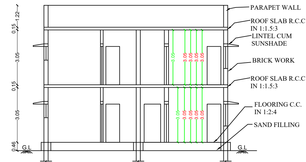
SECTION"A-B"
