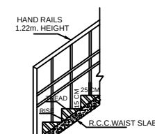
SECTION ON STAIRCASE
