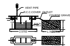
SEPTIC TANK & D-TRENCH DETAILS NOT TO SCALE
