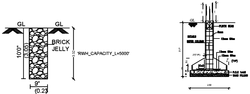
FOUNDATION DETAILS
