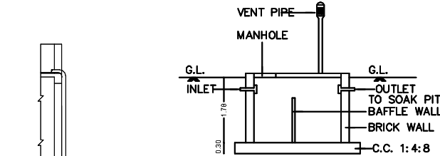
SECTION OF SEP.TANK
