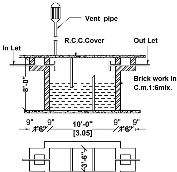
SEPTIC TANK DETAILS (NOT TO SCALE)
