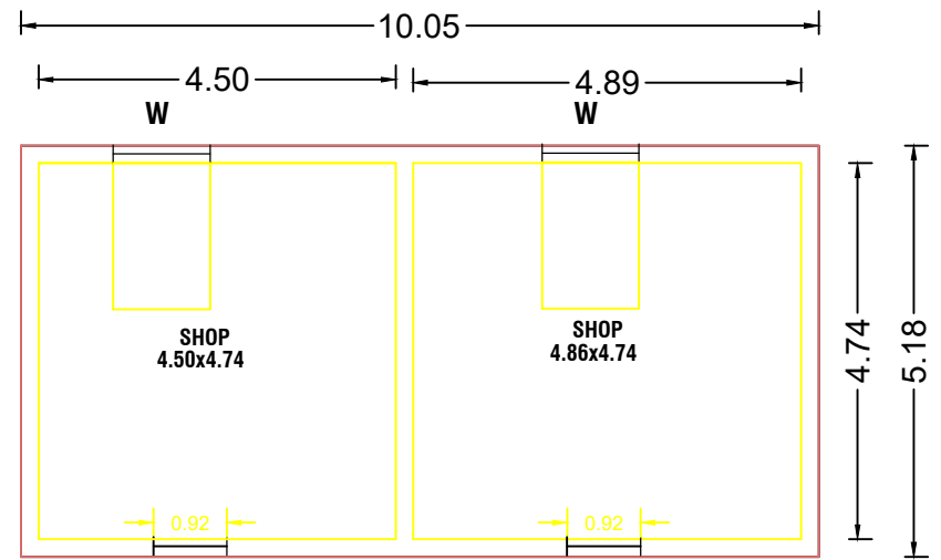
PRO.,GROUND FLOOR PLAN
