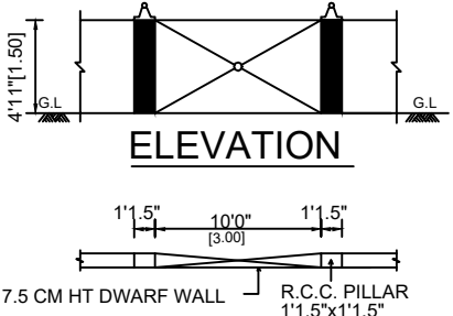
COMPOUND WALL PLAN
