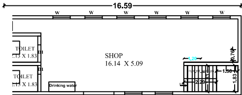
PRO.FIRST FLOOR PLAN
