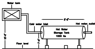
SOLAR WATER HEATER DETAILS
