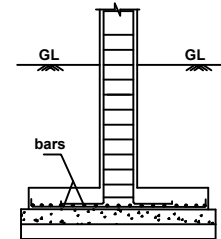
COLUMN DETAILS
