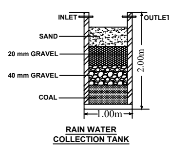
RAIN WATER COLLECTION TANK
