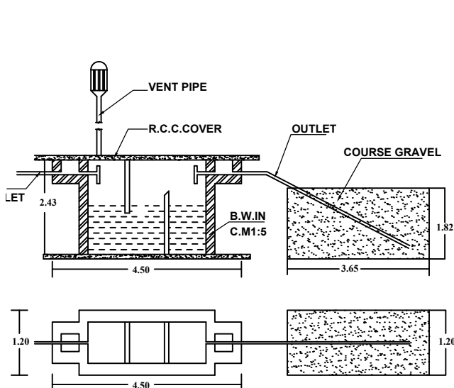
SEPTIC TANK
