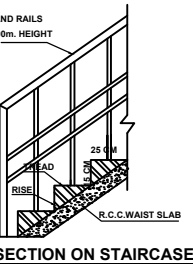
SECTION ON STAIRCASE
