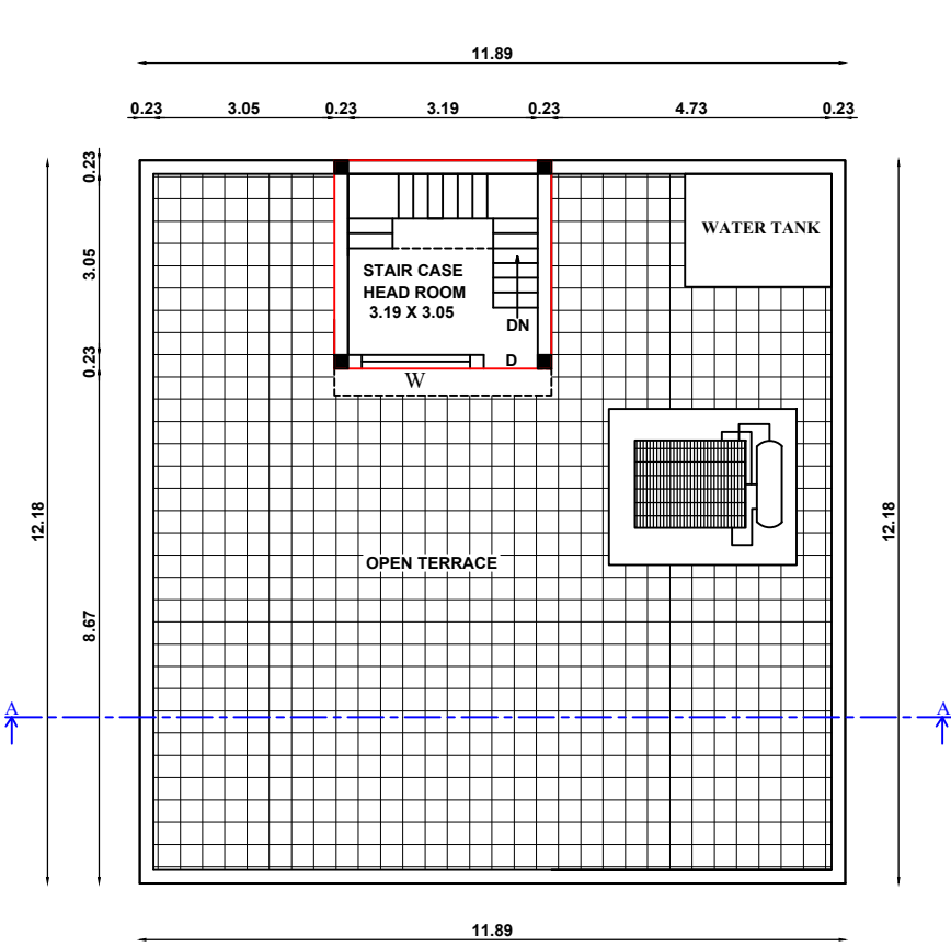
TERRACE/FIRST FLOOR
