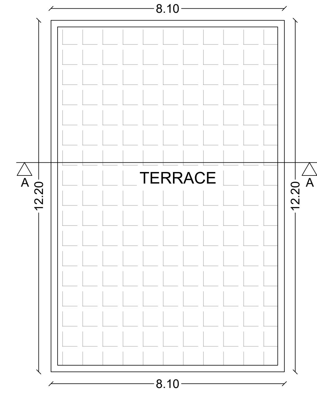
TERRACE FLOOR
