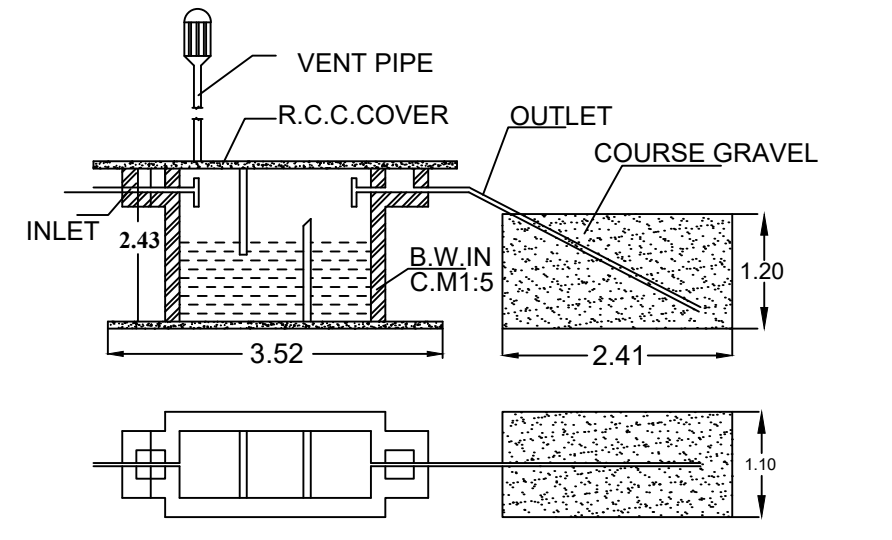
SEPTIC TANK & D-TRENCH DETAILS
