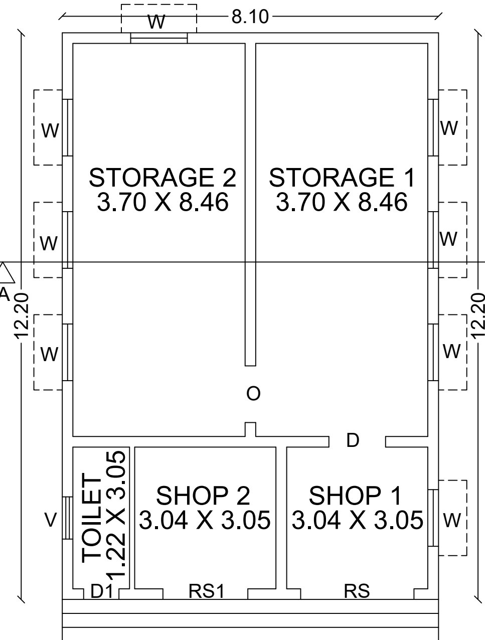
GROUND FLOOR
