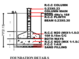
FOUNDATION DETAILS
