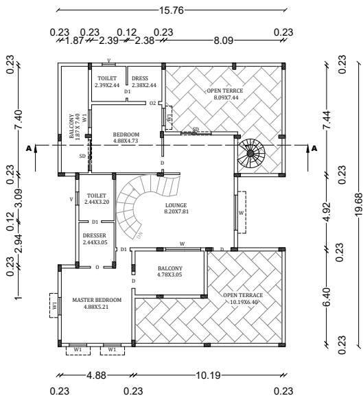
FLOOR - FIRST PLAN
