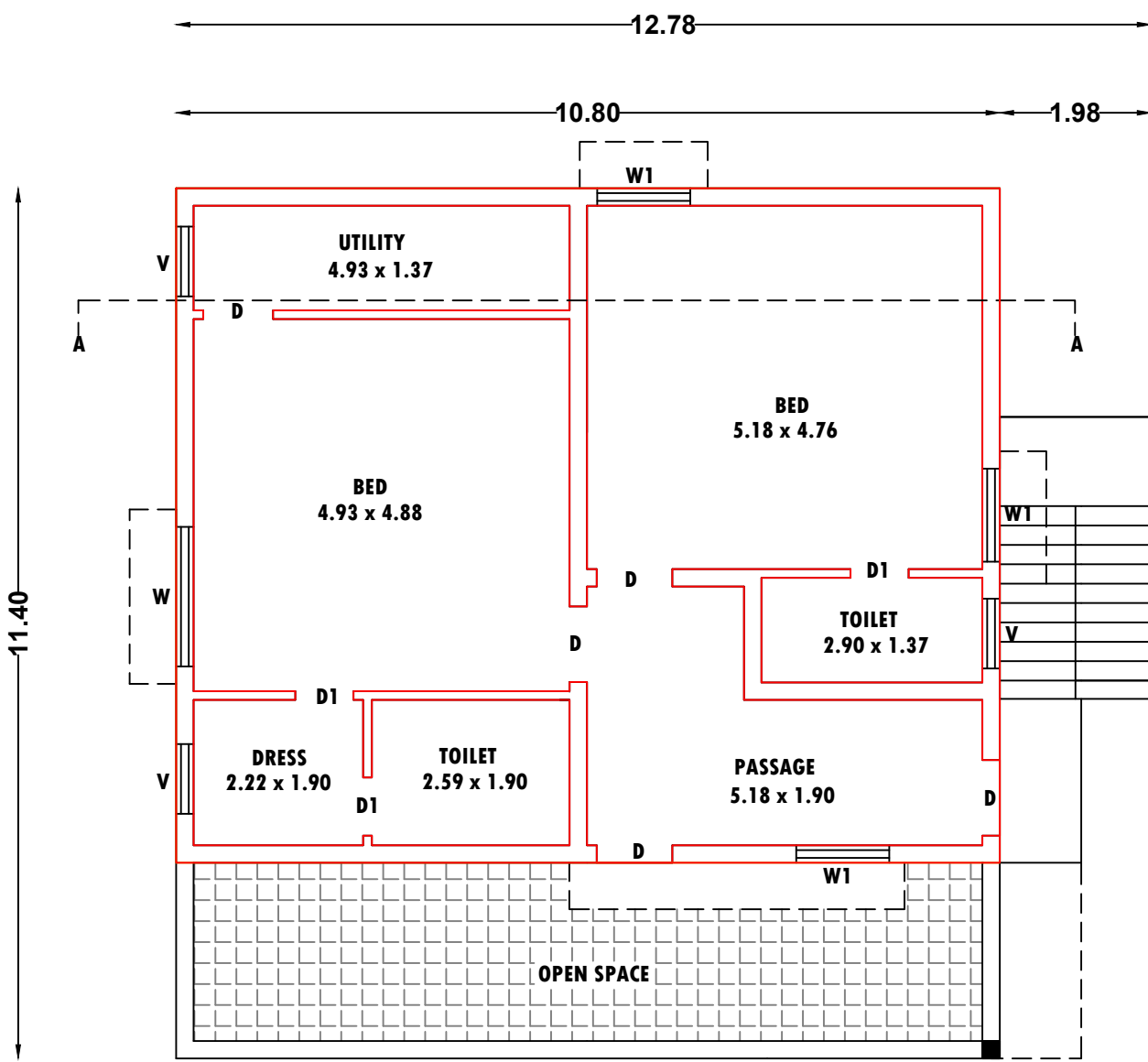
PROPOSED FIRST FLOOR (SCALE 1:100)
