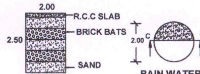
SECTION ON C - D
