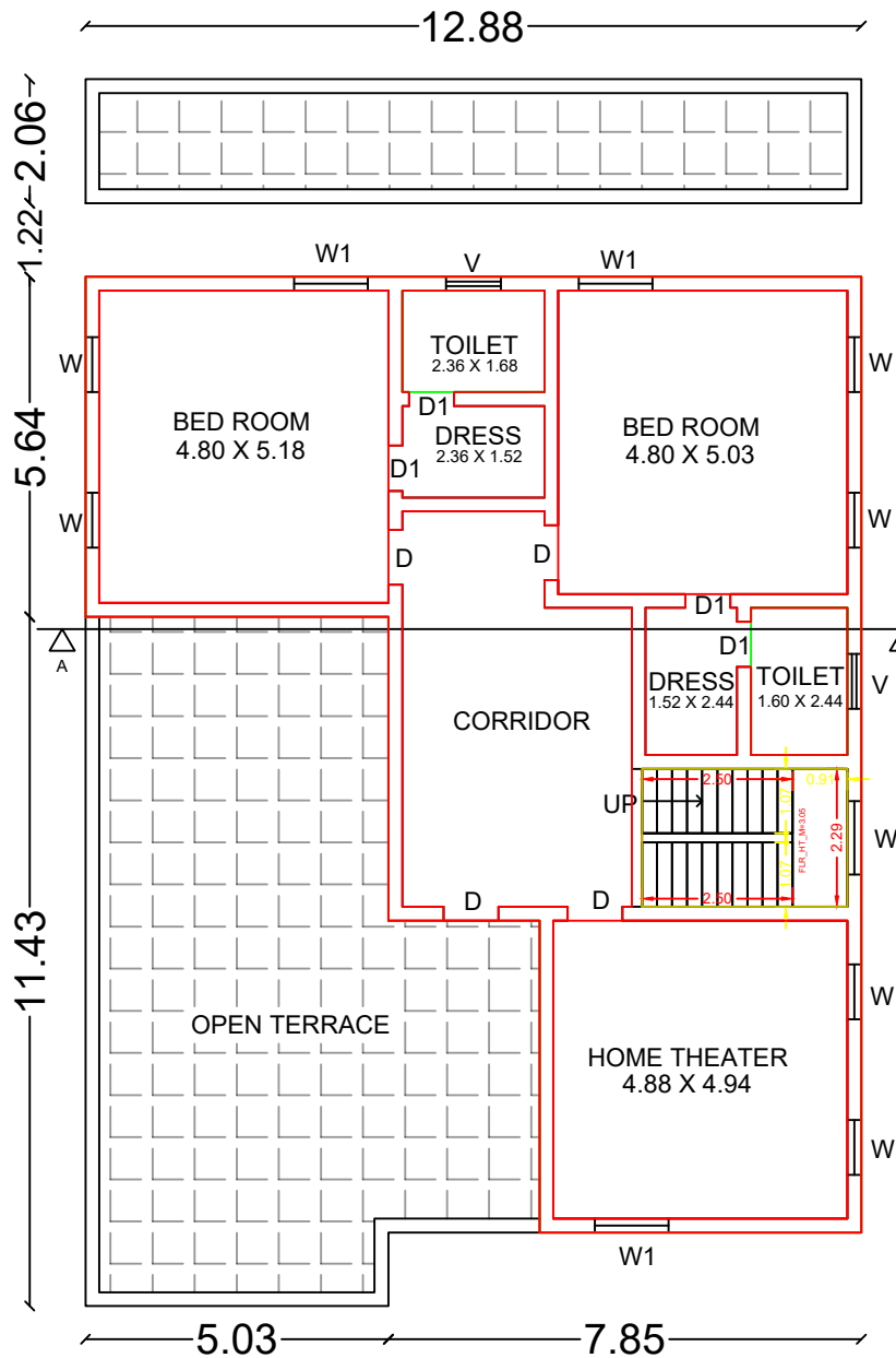
FIRST FLOOR
