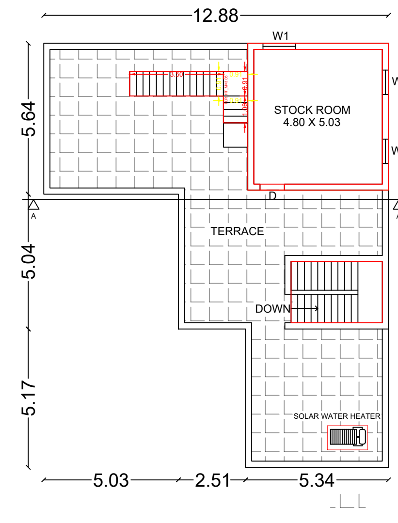
SECOND / TERRACE FLOOR
