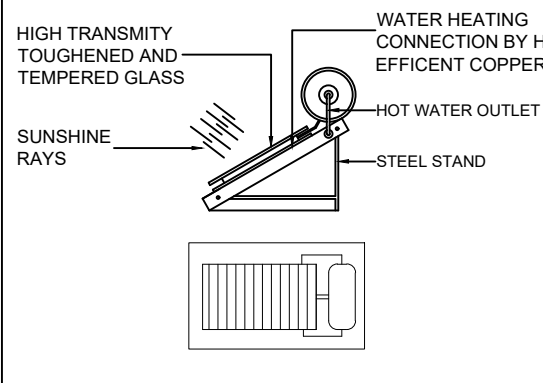
SOLAR HOT WATER SYSTEM DETAIL
