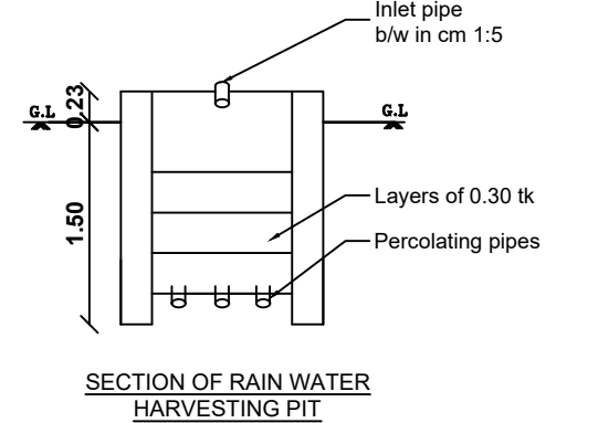
SECTION OF RAIN WATER HARVESTING PIT
