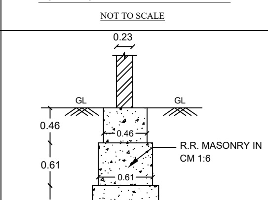
FOOTING DETAIL (NOT TO SCALE)
