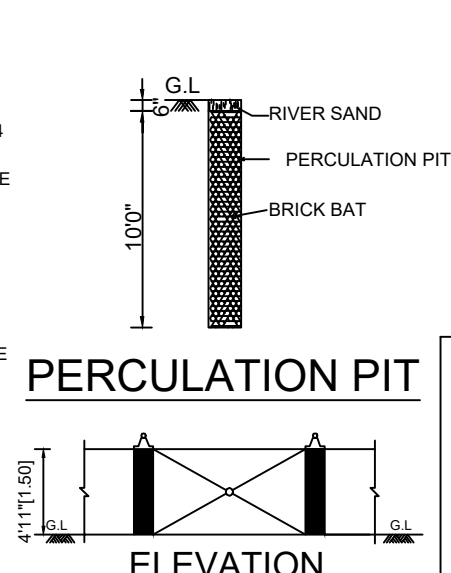
PERCOLATION PIT
