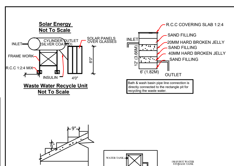
Solar Energy Not To Scale Waste Water Recycle Unit Not To Scale
