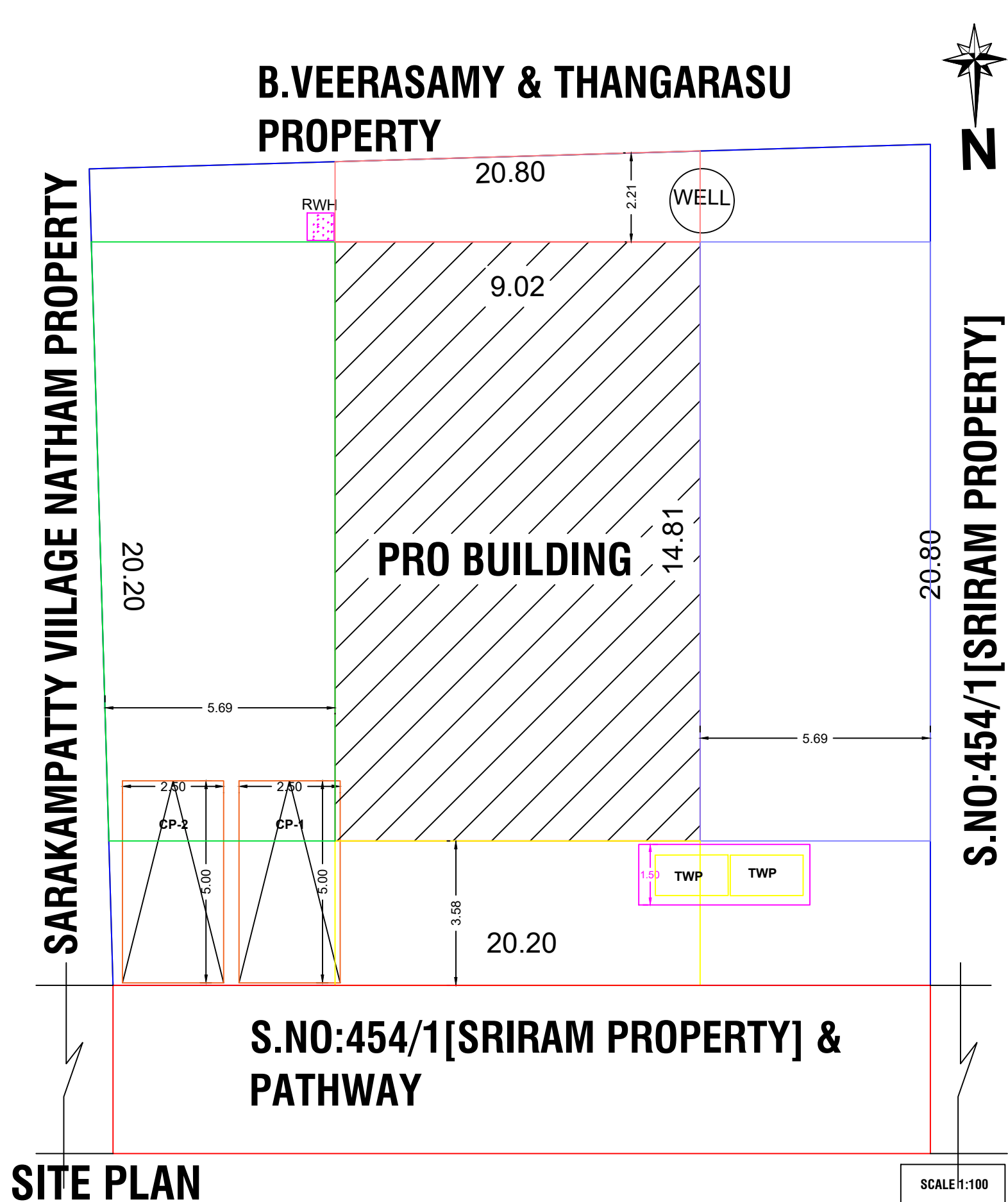
SITE PLAN
