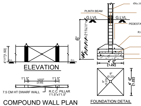
COMPOUND WALL PLAN
