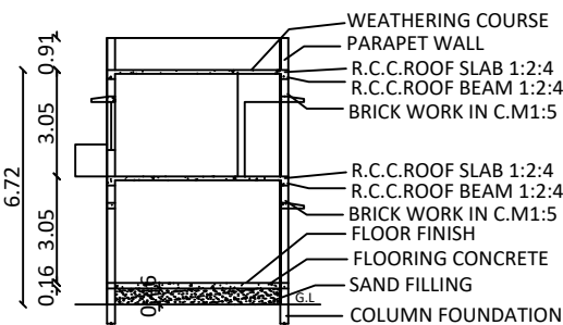
SECTION-SS
