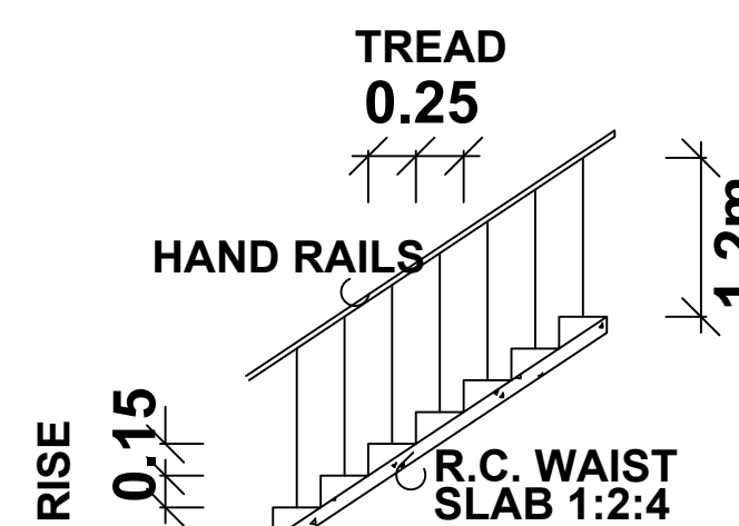
STAIRCASE DETAILS
