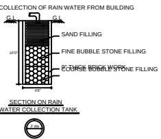
RAIN WATER COLLECTION TANK
