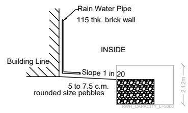
INSIDE Slope 1 in 20 5 to 7.5 c.m rounded size pebbles
