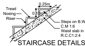
STAIRCASE DETAILS
