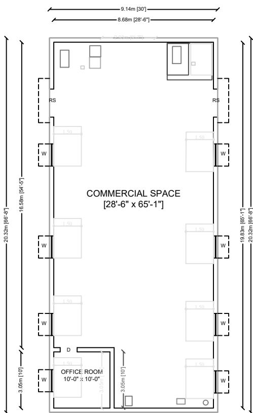
PROPOSED FLOOR PLAN - GROUND FLOOR [USAGE - COMMERCIAL] [FACING - WEST]
