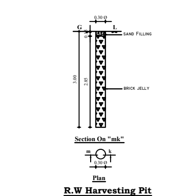
Section On "m-m" R.W Harvesting Pit
