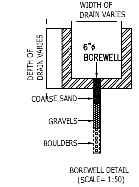
BOREWELL DETAIL (SCALE= 1:50)
