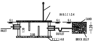
SECTION-AB
