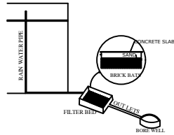
RAIN WATER HVESTING TANK
