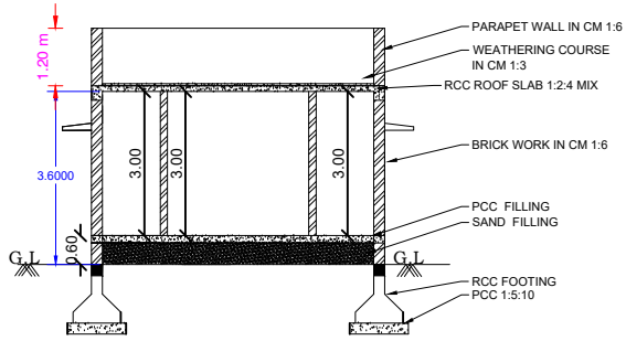
SECTION-"SR"
