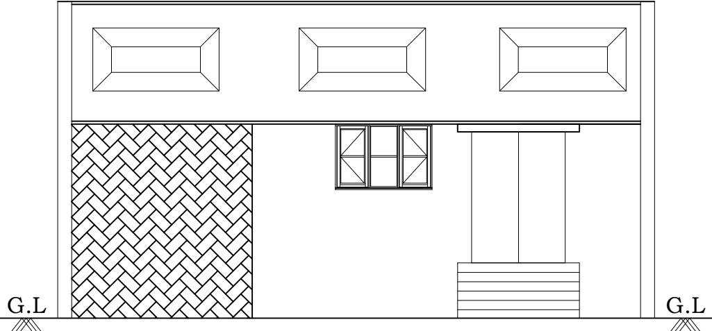
FRONT ELEVATION
