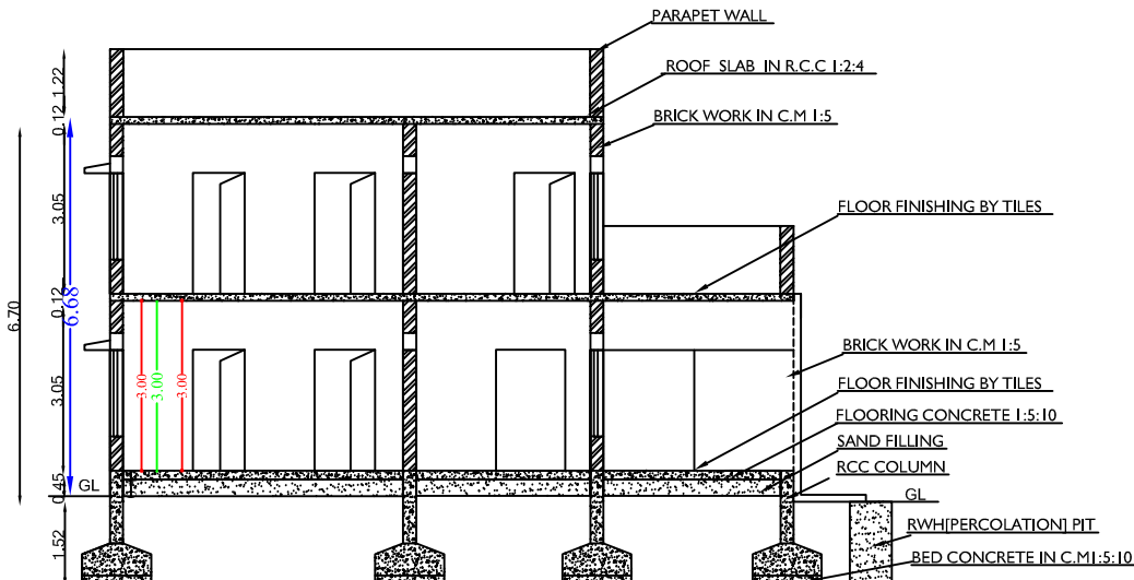
SECTION ON-XY
