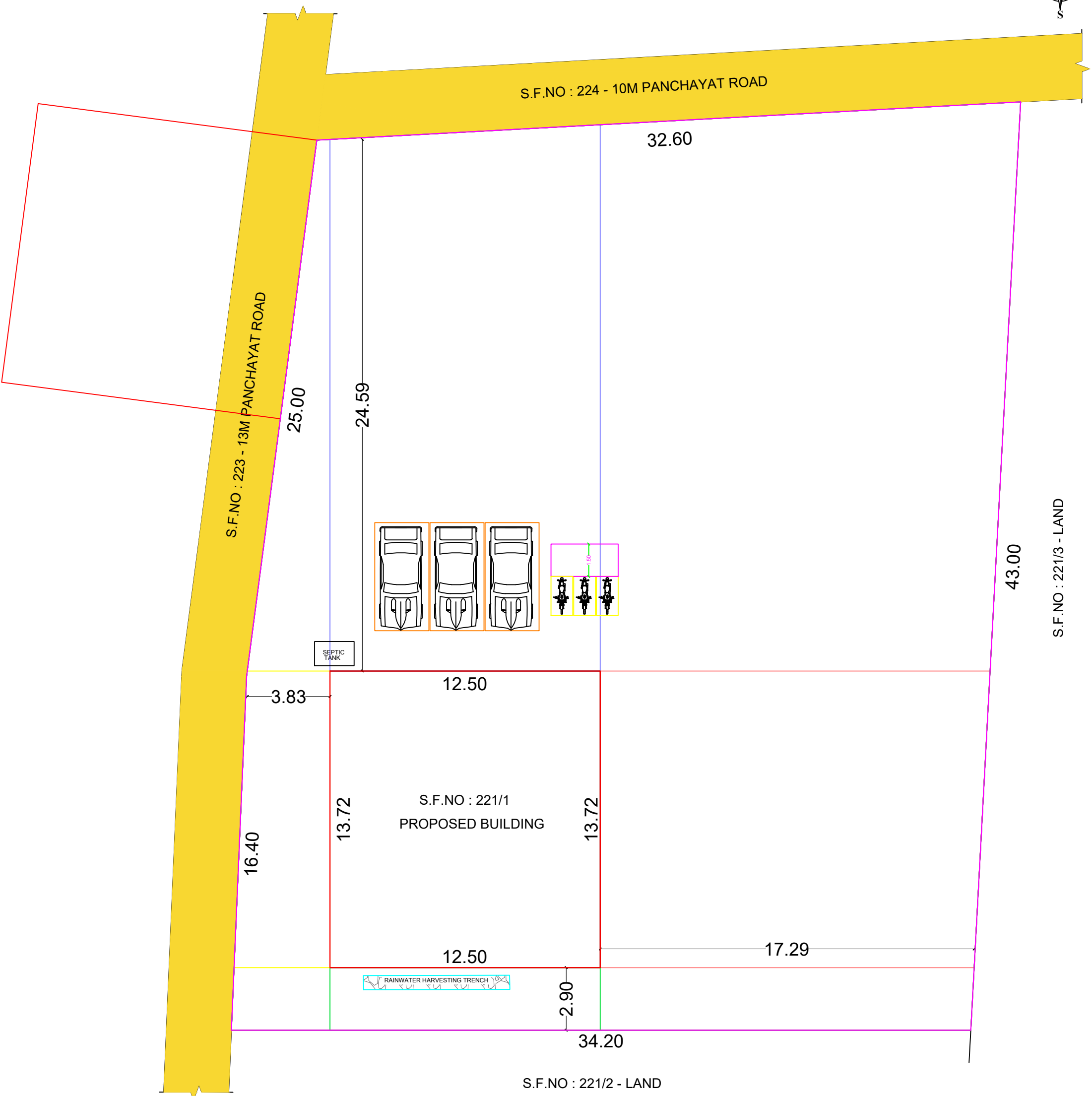
SITE PLAN
