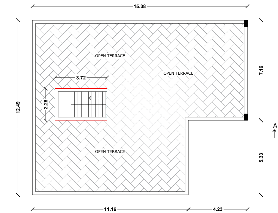
FLOOR - TERRACE PRO. TERRACE FLOOR PLAN
