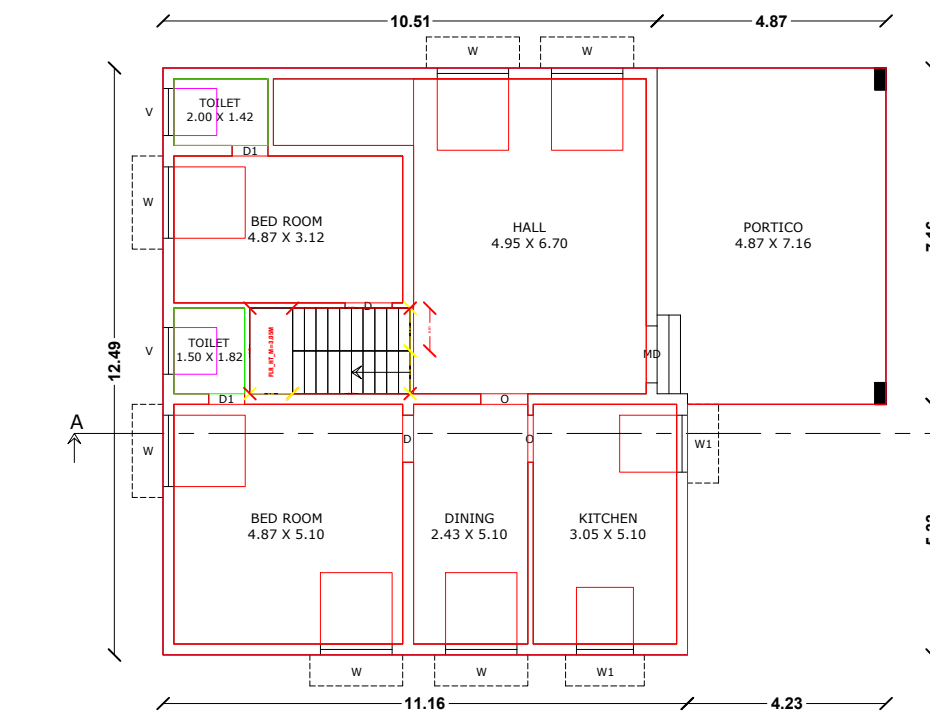
FLOOR - GROUND PRO. GROUND FLOOR PLAN
