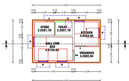
FLOOR-GROUND PRO.GROUND FLOOR PLAN
