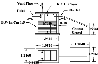
SEPTIC TANK & D-TRENCH DETAILS
