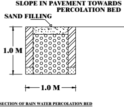
SECTION OF RAIN WATER PERCOLATION BED
