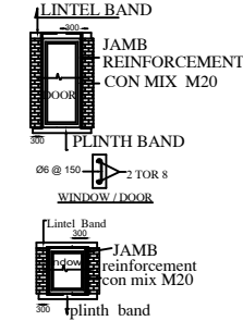
STRUCTURAL PLAN
