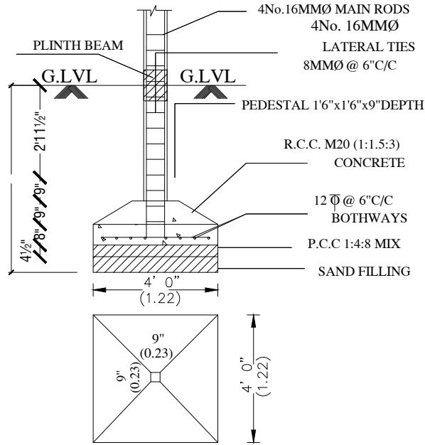
FOUNDATION DETAIL
