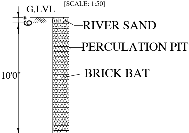
PERCOLATION PIT
