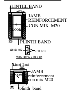
VERTICAL REINFORCEMENT AT JAMBS OF OPENINGS
