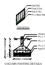
COLUMN FOOTING DETAILS
