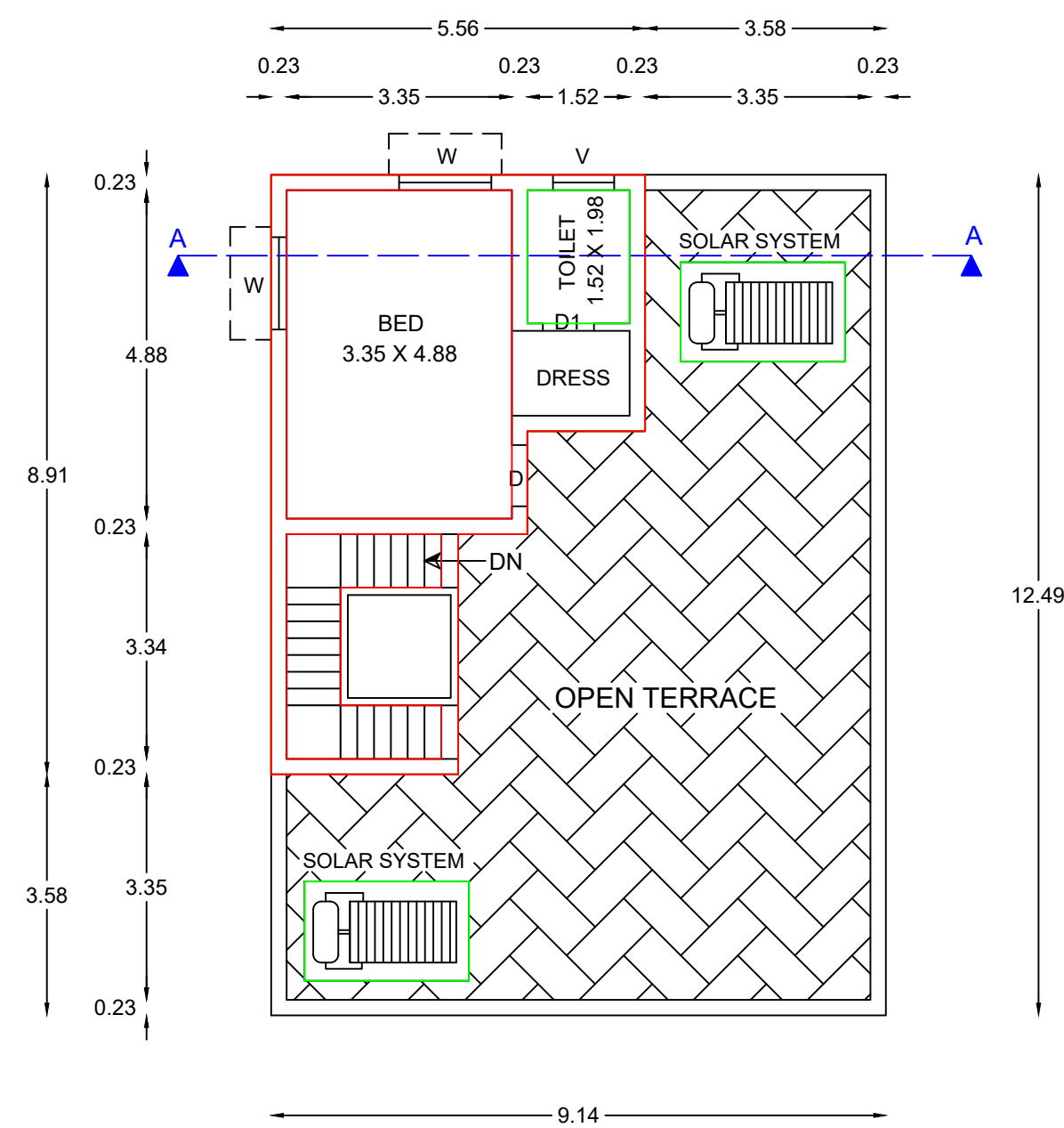
FIRST FLOOR AND TERRACE FLOOR PLAN
