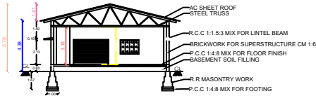
SECTION ON AA
