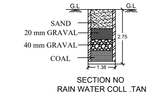
SECTION NO. RAIN WATER COLL. TANK
