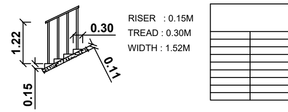
STAIRCASE DETAIL
