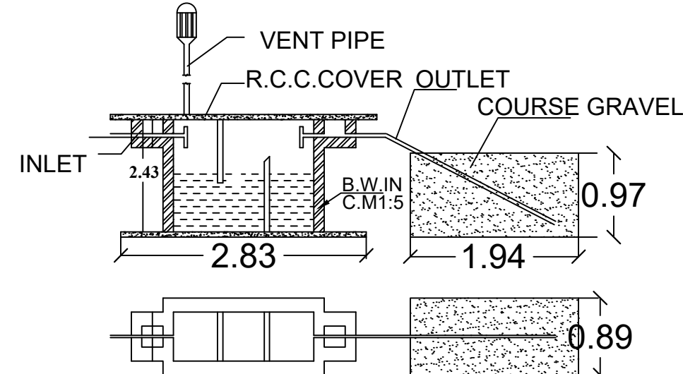
SEPTIC TANK & D-TRENCH DETAILS
