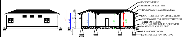
FRONT ELEVATION WEST SIDE
