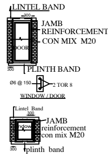
VERTICAL REINFORCEMENT AT JAMBS OF OPENINGS
