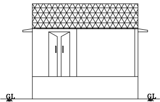
FRONT ELEVATION
