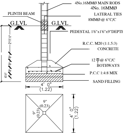
FOUNDATION DETAIL
