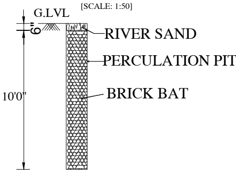
PERCOLATION PIT
