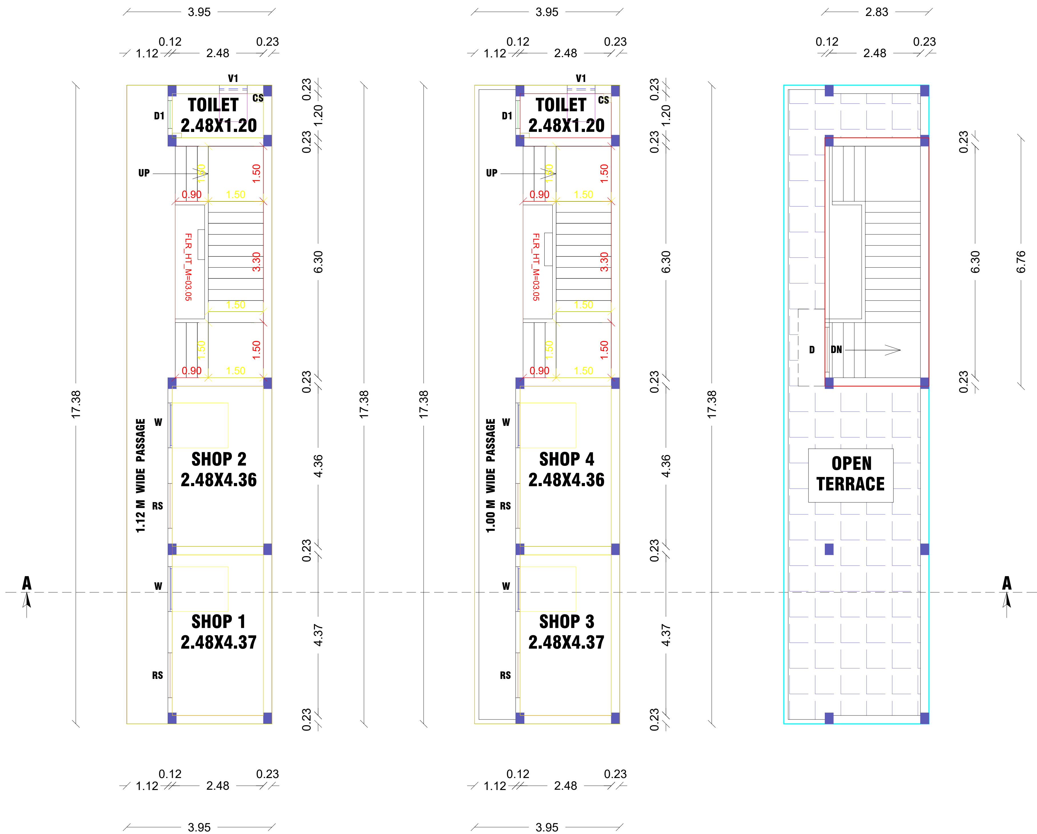
LOOR-GROUND
