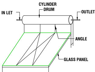
SOLAR LIGHT SYSTEM
