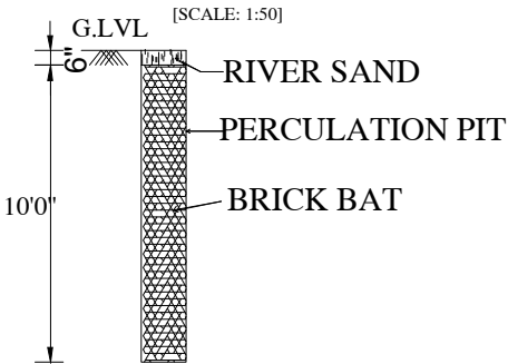
PERCOLATION PIT
