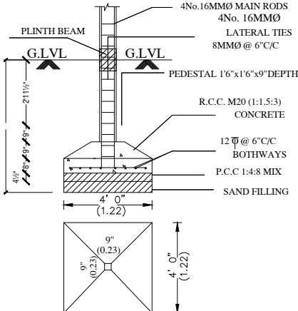
FOUNDATION DETAIL
