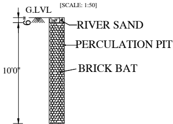
PERCOLATION PIT
