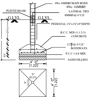
FOUNDATION DETAIL
