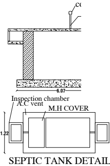
SEPTIC TANK DETAILS
