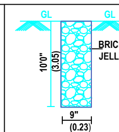
PERCULATION PIT
