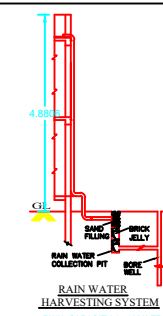
RAIN WATER HARVESTING SYSTEM
