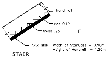
STAIR
