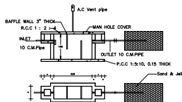
SEPTIC TANK AND TRENCH
