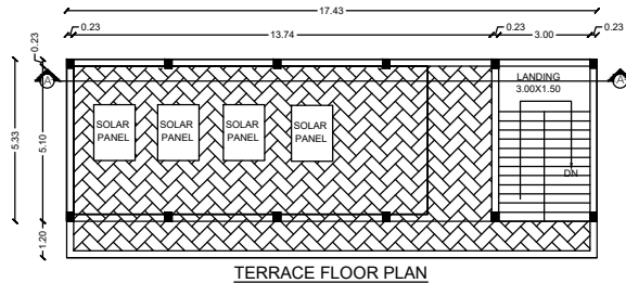
TERRACE FLOOR PLAN
