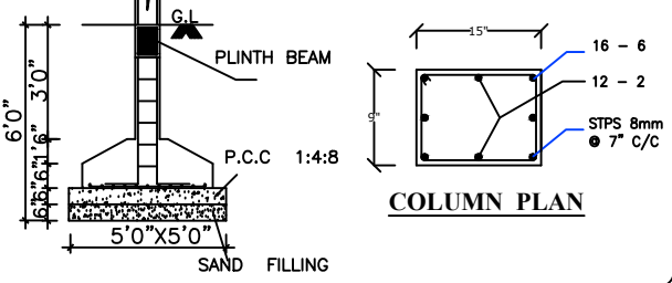
DETAILS OF COLUMN FOOTING FOUNDATION SCALE 1"-4'0"
