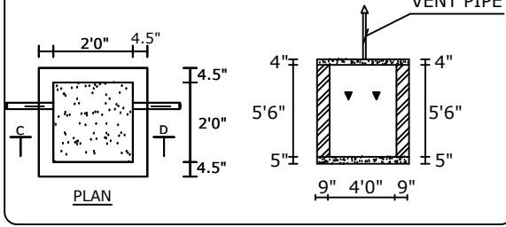
RAIN WATER HARVESTER NOT TO SCALE
