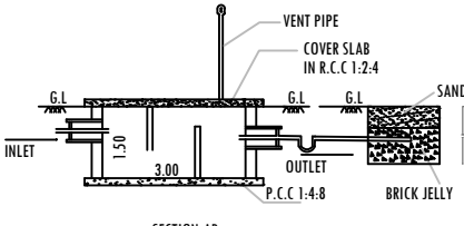
SECTION-AB
