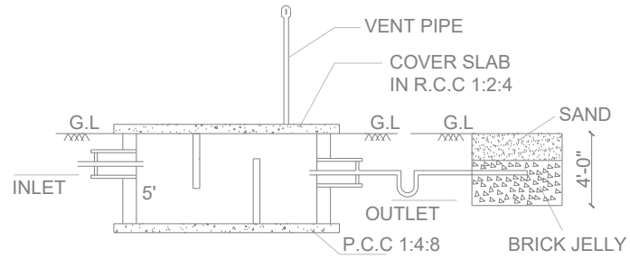
SECTION-AB
