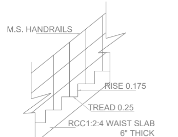
STAIRCASE DETAILS SCALE- 1:20
