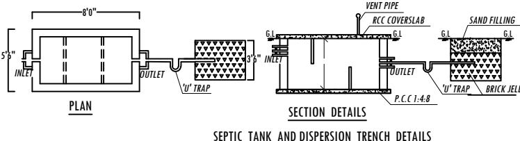
SEPTIC TANK AND DISPERSION TRENCH DETAILS
