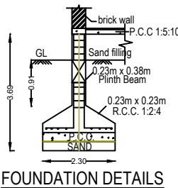
FOUNDATION DETAILS
