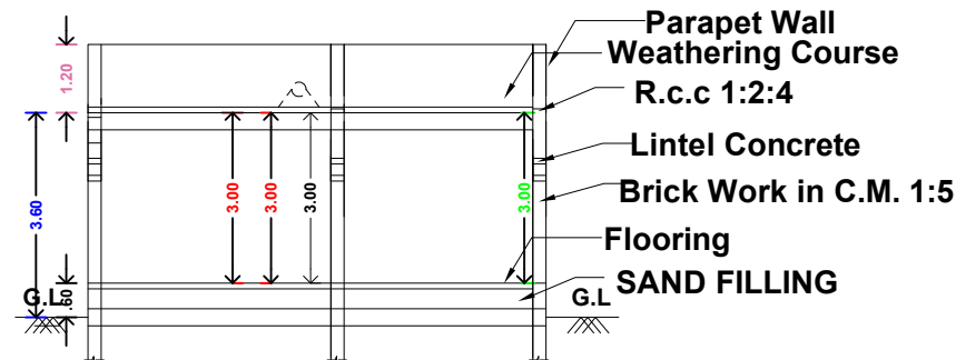
SECTION ON "BB"
